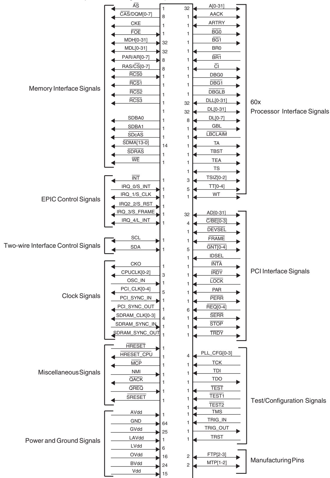
Figure 3-1. PC107A Microprocessor Signal Groups
