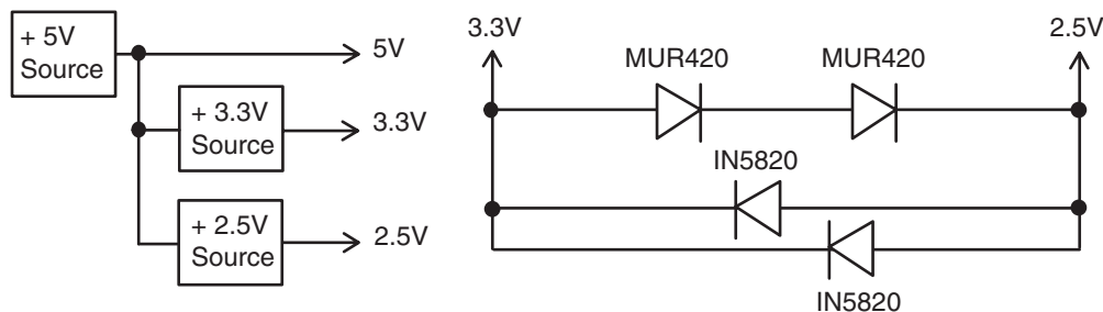
Figure 10-2. Example Voltage Sequencing Circuits
