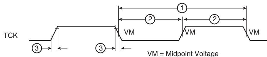
Figure 7-16. JTAG Clock Input Timing Diagram
