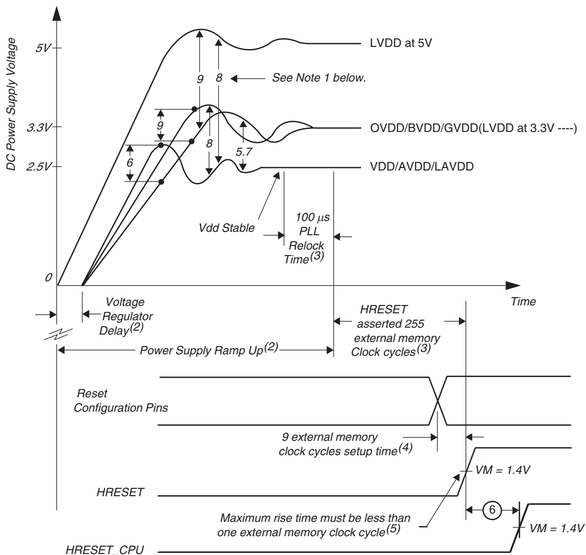
Figure 5-1. Supply Voltage Sequencing and Separation Cautions
