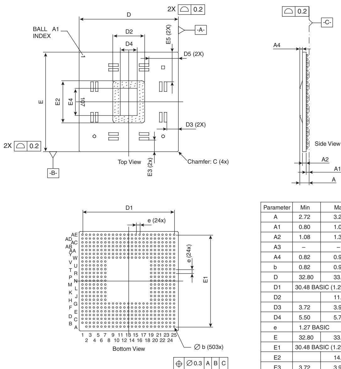
Figure 9-2. Mechanical Dimensions and Bottom Surface Nomenclature of the 503-ball HiTCE CBGA Package
